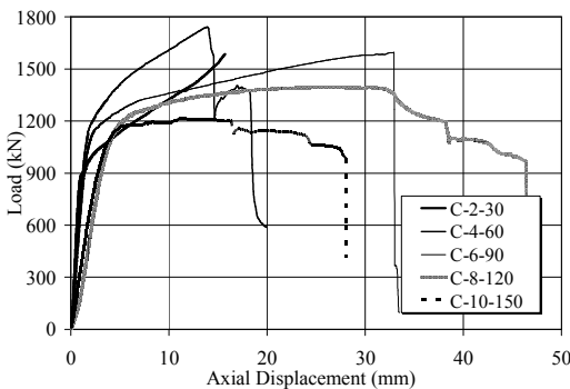
Figure 6. Load- axial deformation relationship.
