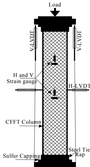
Figure 2. Test setup.
