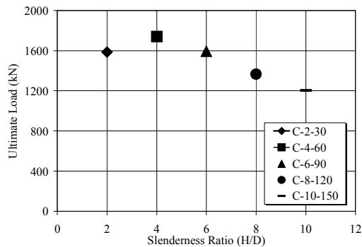
Figure 5. Load-slenderness ratio relationship.
