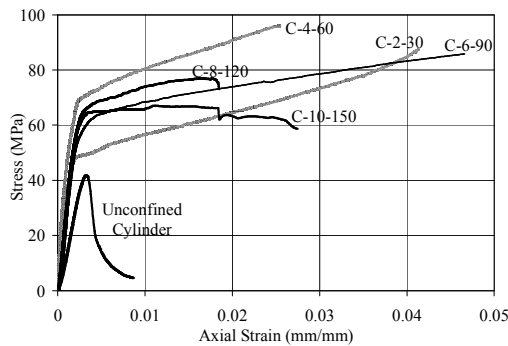
Figure 4. Stress-strain relationship.
