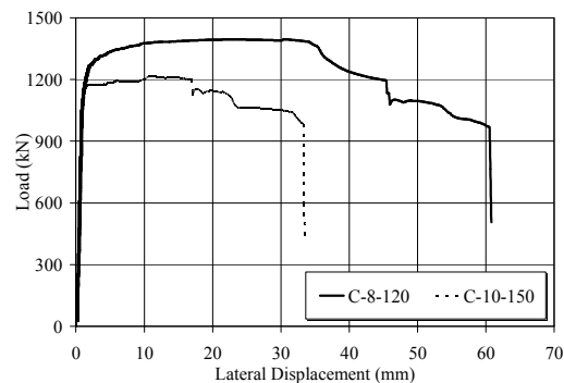
Figure 7. Load-lateral deformation relationship.
