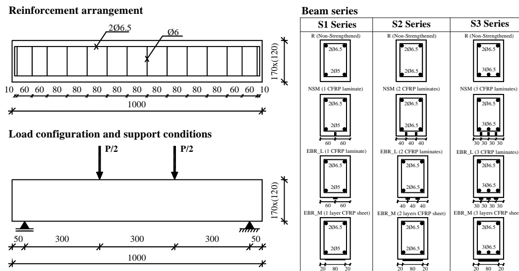
Figure 1. Beams used for analytical and numerical analysis.
