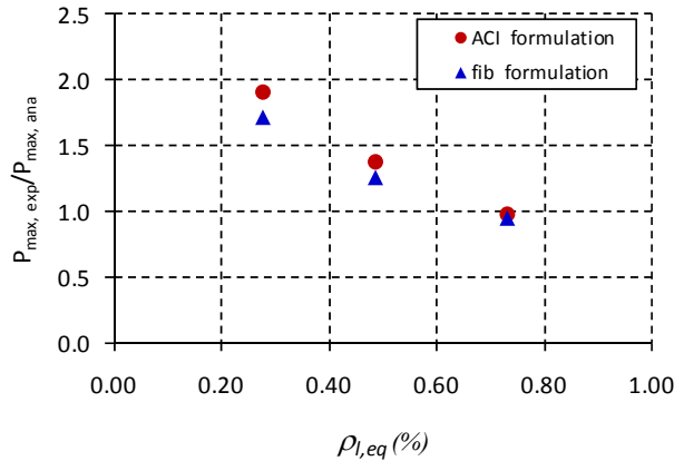
Figure 3. Relationship between P_{max}^{exp}/P_{max}^{ana} and \rho_{l,eq} for the beams with NSM laminates.
