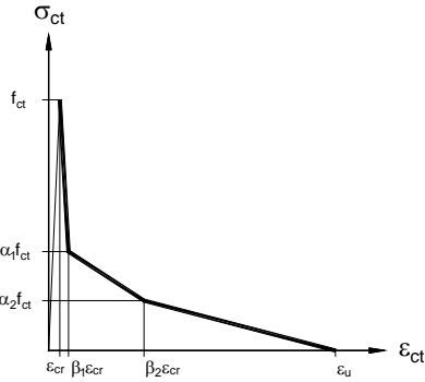
Figure 4. Trilinear stress-strain diagram to model the concrete post-cracking behaviour.
